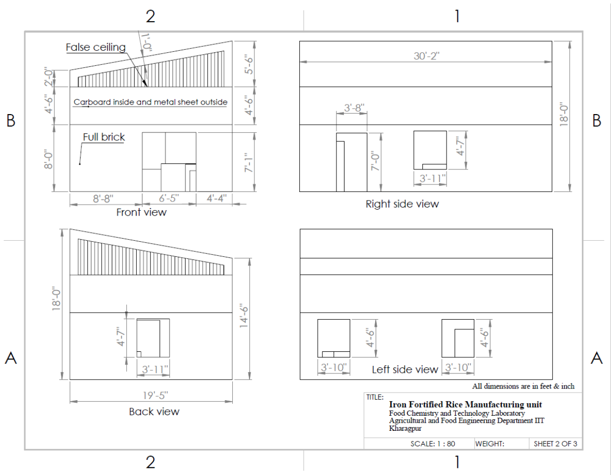
Fig. 2: 2D views of the IFRMU indicating position of doors & windows
