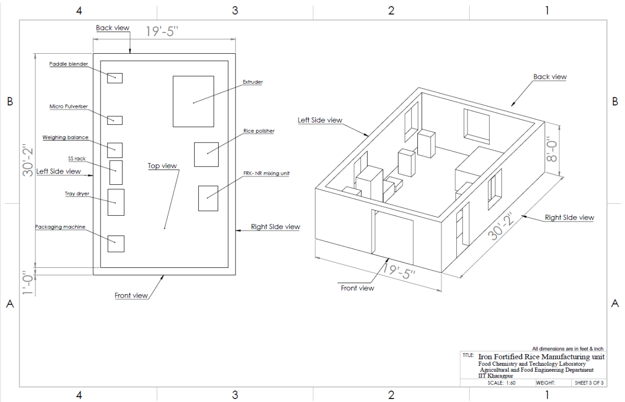
Fig. 3 Positions of existing installed equipment inside the IFRMU
