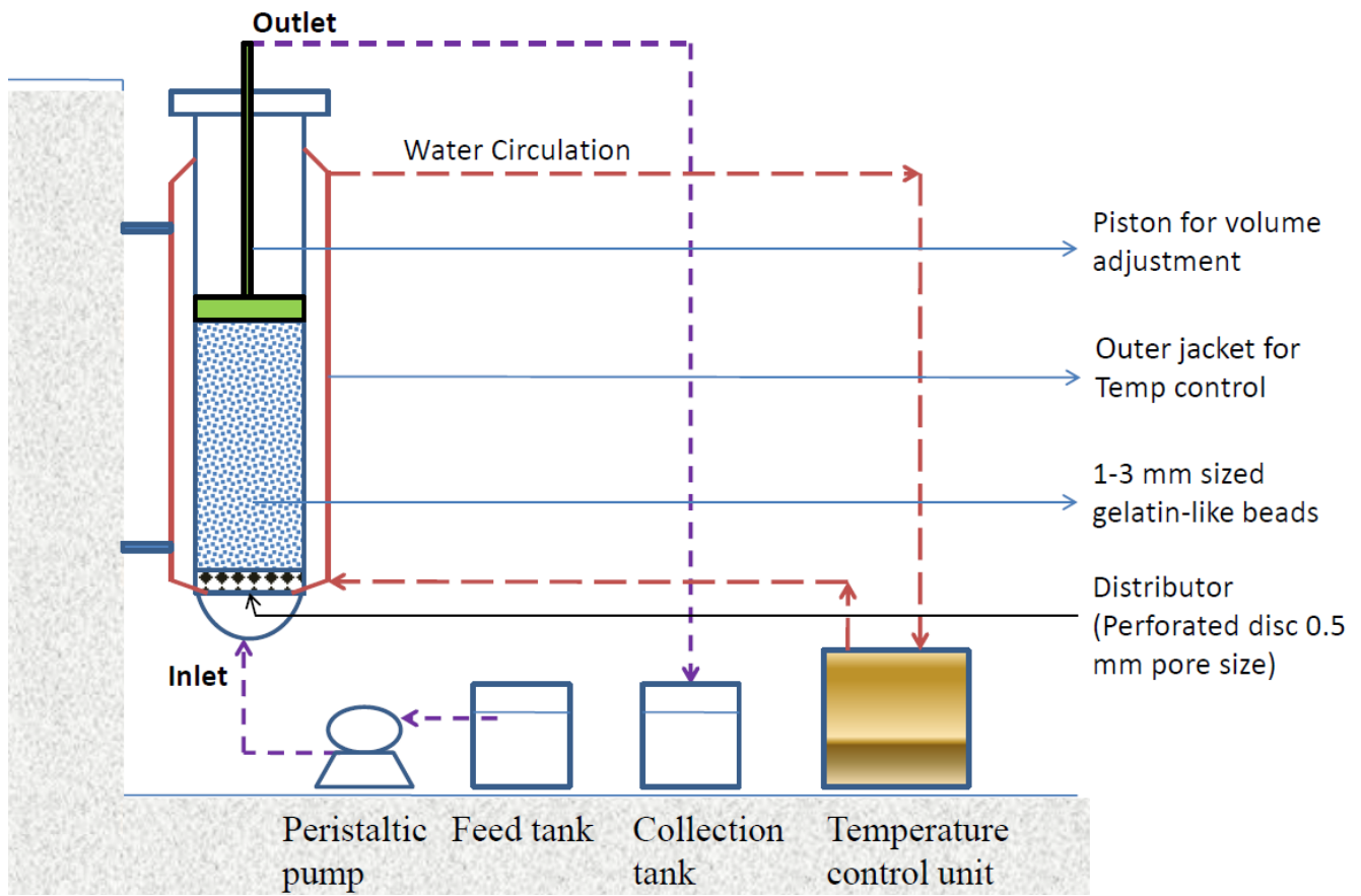
Schematic Diagram of the Paacked Bed Reactor Set-up
