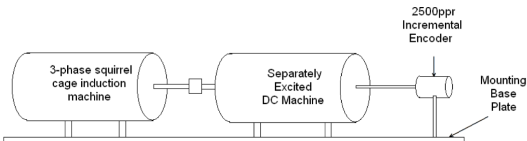
Simplified schematic diagram of the full unit.
