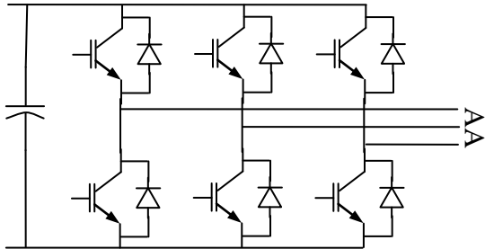
Circuit diagram of one basic unit
