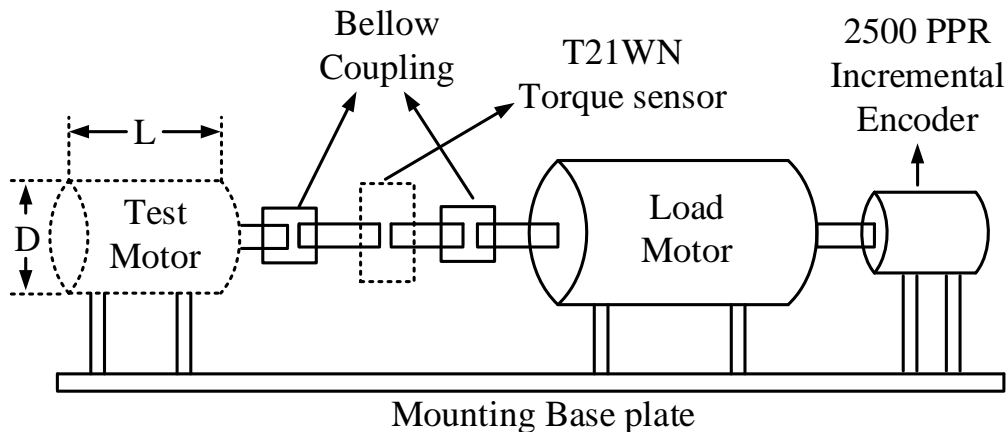
Fig: Motor test bench to be developed at IIT Kharagpur (items with dotted lines will be provided by IIT KGP)
